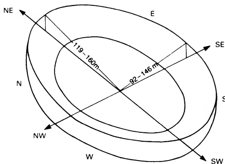
6 Viewing distance determines the stadium size
